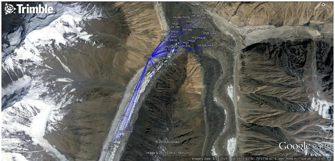
Figure 23. GNSS Survey measuring points as visualised by the Trimble TSC3 controller and Google Earth.
